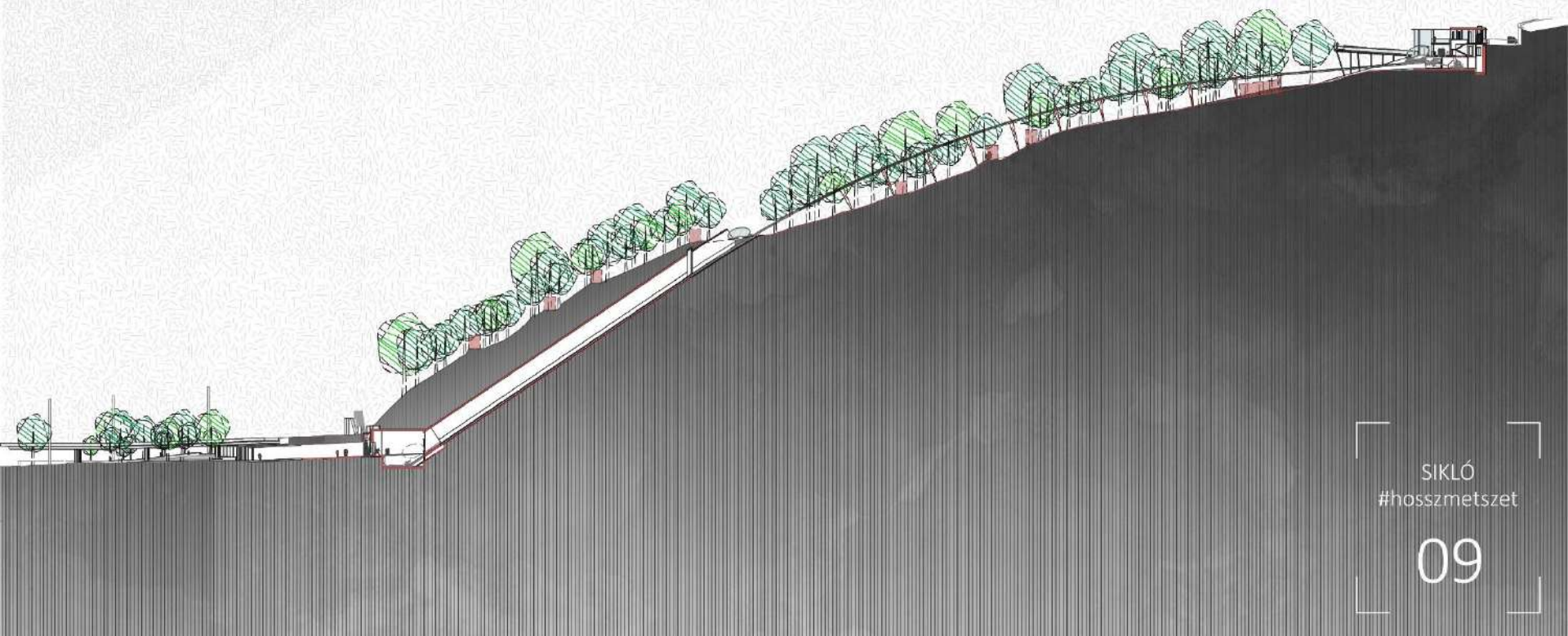
Section of the planned Gellért hill funicular
